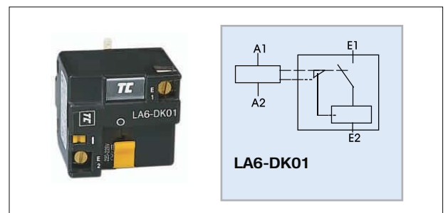
Latch Add-on Block (Front mounted) LA6-DK01
