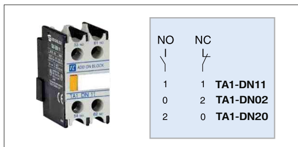
Auxiliary Contact Block (Front mounted) TA1-DN
